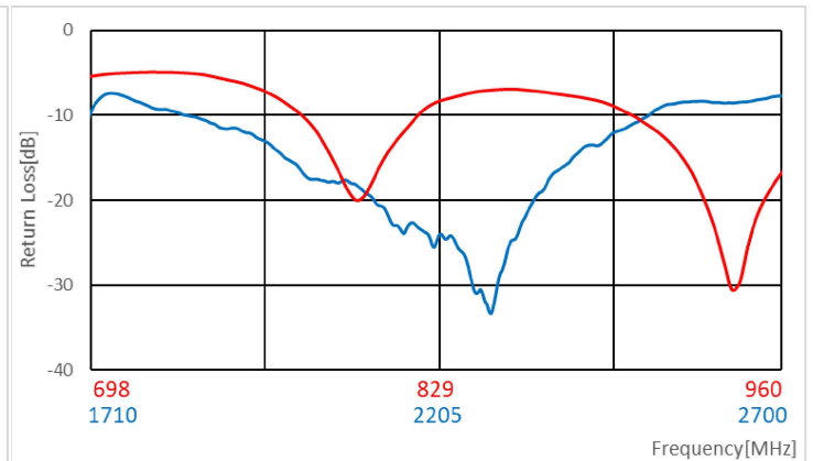
Return Loss
